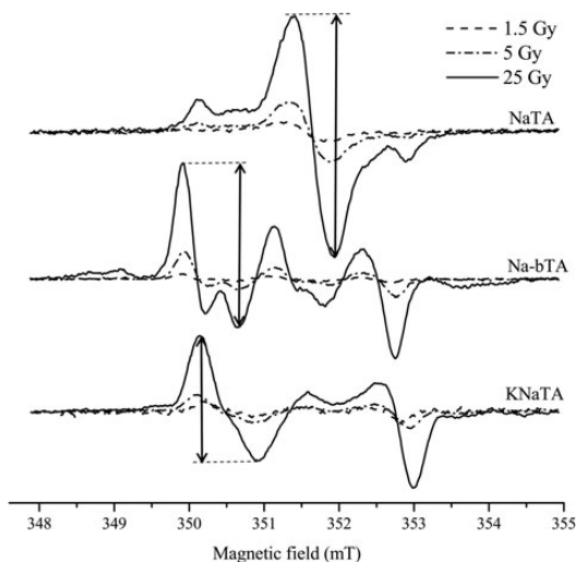
Figure 1. ESR spectra of sodium tartrates compounds normalised to the mass of the samples irradiated at three different radiation doses.
