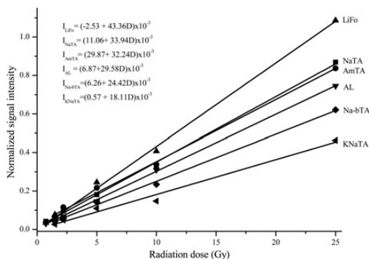
Figure 3. Calibration dose–response curves of interested samples (filled squares, NaTA; filled diamonds, Na-bTA; filled side triangles, KNaTA); filled circles, AmTA; filled triangles, LiFo; filled inverted triangles, AL.
